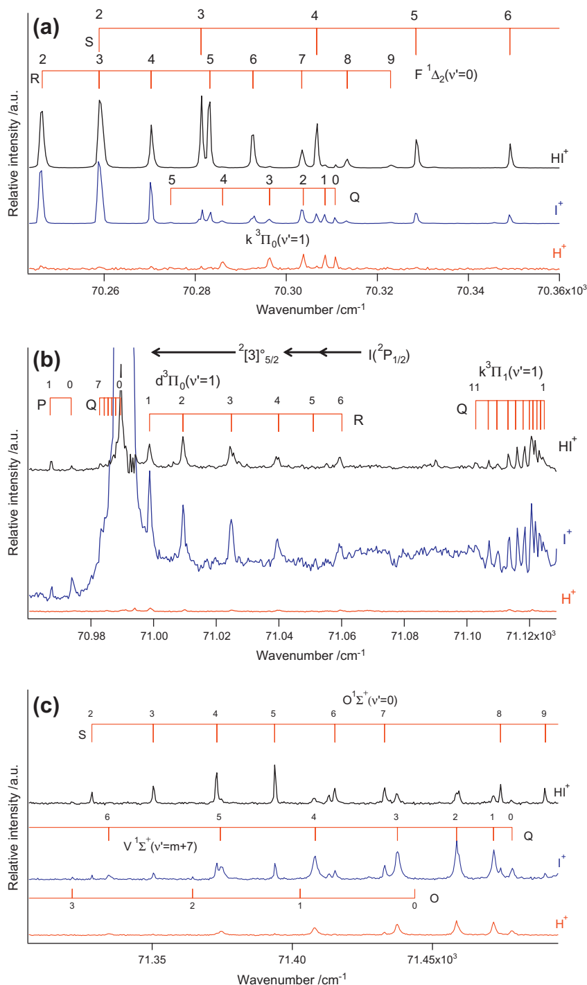
Fig. 2. 1D-REMPI spectra for H + , I + , and HI + and I ' assignments of rotational peaks corresponding to two-photon resonance excitations to F 1 Δ 2 (v' = 0) (a), d 3 Π 0 (v' = 1) (b), k 3 Π 1 (v' = 1) (b), O 1 Σ + (v' = 0) (c), V 1 Σ + (v' = m + 7) (c), V 1 Σ + (v' = m + 8) (d and e), I 1 Δ 2 (v' = 0) (d), and V 1 Σ + (v' = m + 9) (d and e). In Fig. 2e, the H + spectrum from Fig. 2d is intensified to show the presence of the ion-pair states V 1 Σ + (v' = m + 7) and V 1 Σ + (v' = m + 8) more clearly.
